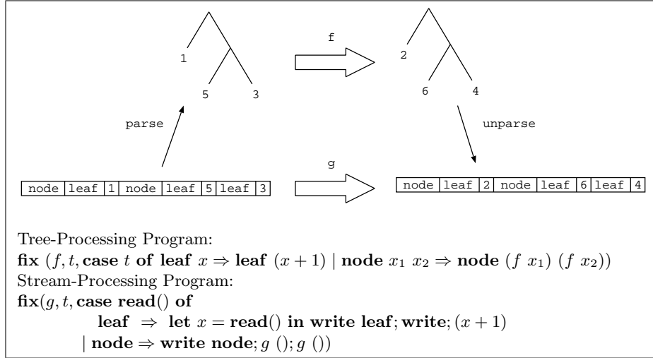
Fig. 1. Tree-processing and stream-processing
